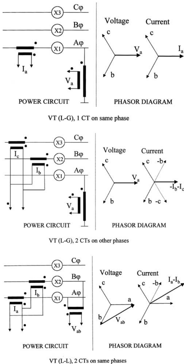
FIGURE 3.7.2 Phasing of voltage and current inputs.
