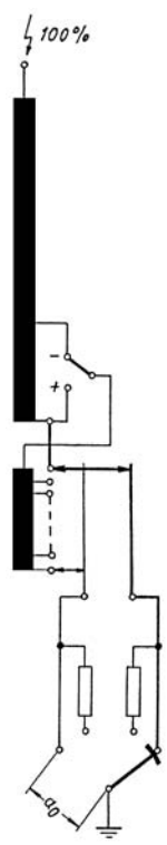
FIGURE 3.3.21 Voltage stress between selected and preselected tap of coarse-tap winding arrangement, LTC in mid-position.
