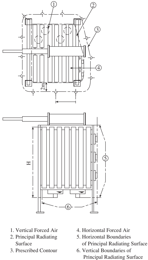
FIGURE 3.9.3 Typical microphone positions for sound measurement on cooling auxiliaries mounted on a separate structure spaced \geq 3 m from the principal radiating surface of the transformer. (From IEC 60076-10. With permission.)
