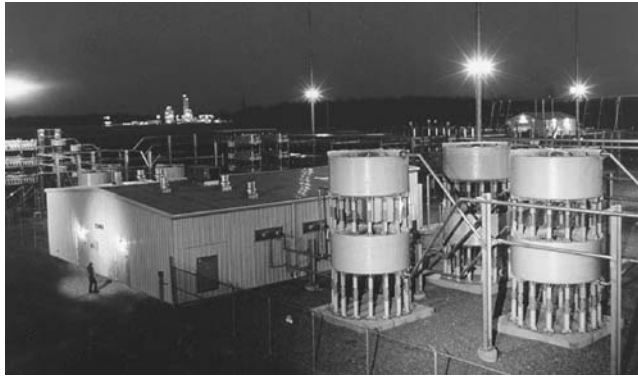
FIGURE 2.9.23 34-kV, 25-MVAR (per phase) thyristor-controlled reactors.
