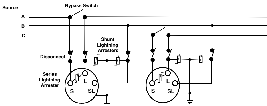
FIGURE 2.7.7 Connection of two voltage regulators regulating a three-phase, three-wire wye or delta circuit.
