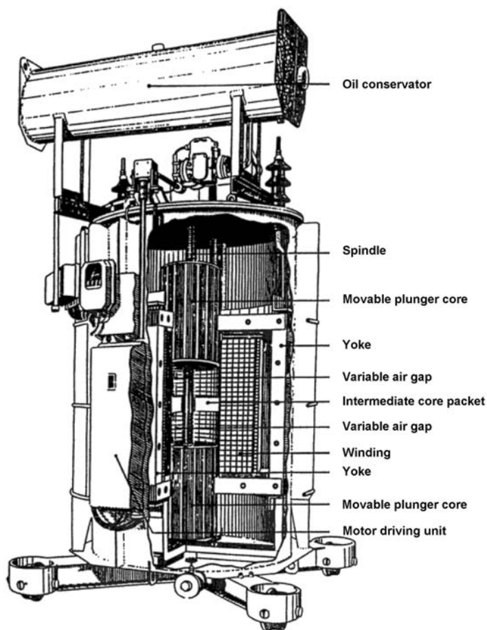
FIGURE 2.9.11 Arc-suppression reactor.
