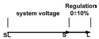
FIGURE 2.7.4 Phasor diagram of a voltage regulator regulating a single-phase circuit.
