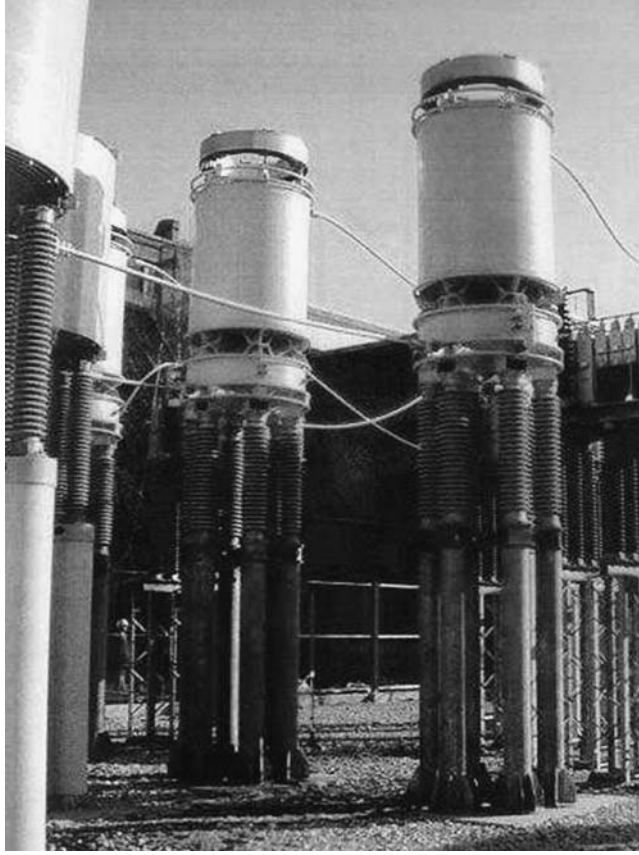
FIGURE 2.9.39 Tapped filter reactor with de-Q'ing rings.
