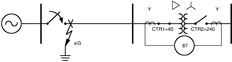
FIGURE 3.8.18 Transformer energization while A-phase is faulted.
