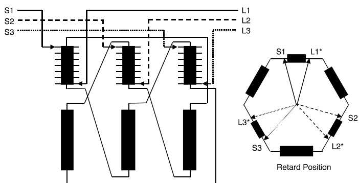
FIGURE 2.3.11 Delta-hexagonal PST.
