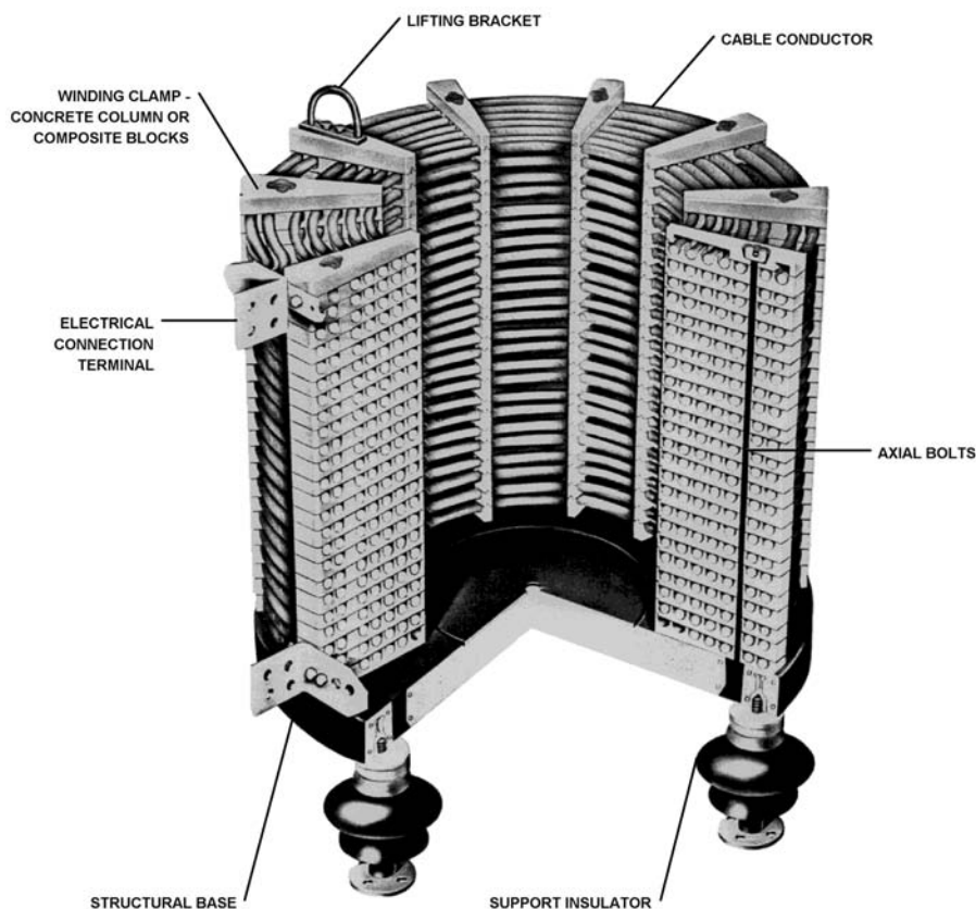
FIGURE 2.9.1 Open-style reactor.
