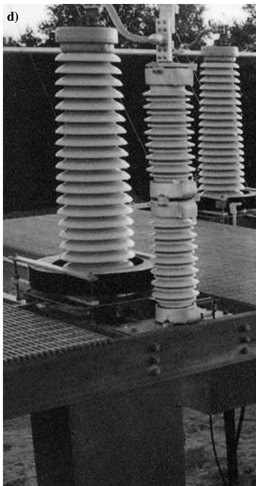
FIGURE 2.6.20 (a) Small 600-V-class window-type CT mounted over a bushing on a 15-kV recloser. (b) 15-kV-class window-type CTs with porcelain sleeve mounted on substation structure. (c) 600-V-class window-type CTs mounted over a 15-kV bus inside a metal enclosure. (d) Large 600-V-class window-type CT (slipover) mounted over a high-voltage bushing. (e) 8.7-kV-class window-type CT with rectangular opening. (Photos courtesy of Kuhlman Electric Corp.)
