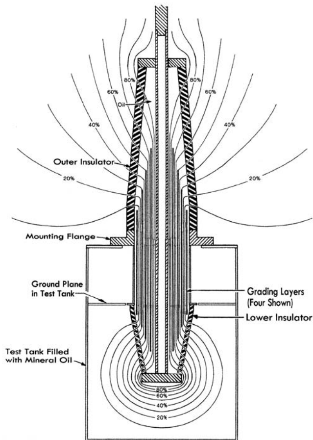
FIGURE 3.2.3 Exponential plot of oil-filled, capacitance-graded bushing.
