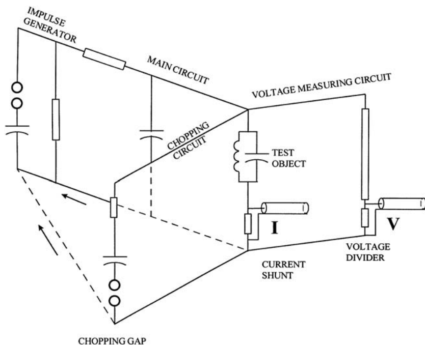
FIGURE 3.6.8 Impulse-test setup.
