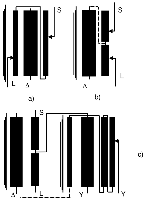
FIGURE 2.3.14 Quadrature booster set (300 MVA, 50 Hz, 400\pm12\cdot1.25\%/115\pm12\cdot1.45^\circ kV).
