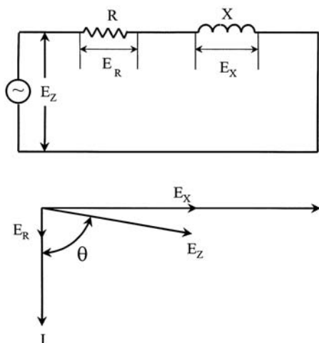
FIGURE 3.6.16 Equivalent circuit and phasor diagram for load-loss test.
