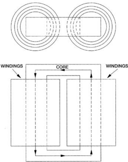
FIGURE 2.1.3 Schematic of single-phase core-form construction.
