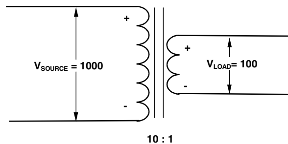
FIGURE 2.7.12 Transformer with 10:1 turns ratio.
