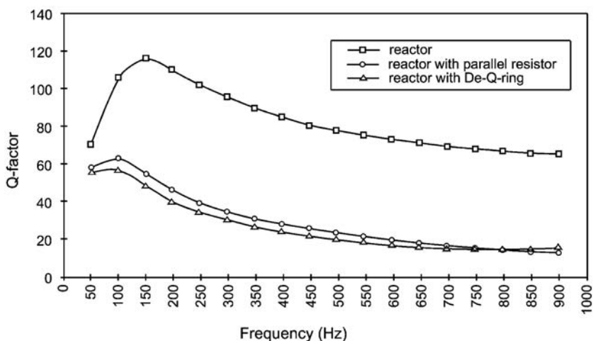
FIGURE 2.9.42 Graph of Q vs. frequency for a natural Q-filter reactor, a filter reactor plus parallel resistor, and a filter reactor with a de-Q'ing system.
