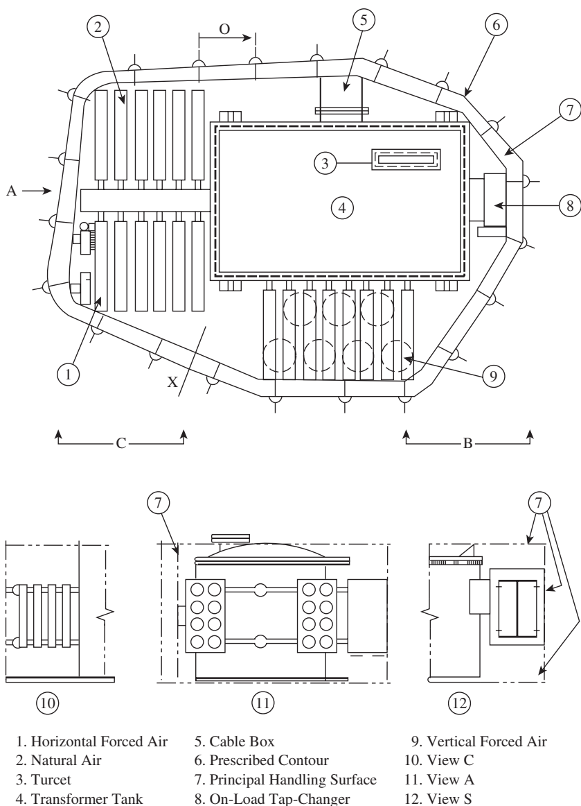
FIGURE 3.9.2 Typical microphone positions for sound measurement on transformers having cooling auxiliaries mounted either directly on the tank or on a separate structure spaced <3 m from the principal radiating surface of the main tank. (From IEC 60076-10. With permission.)
