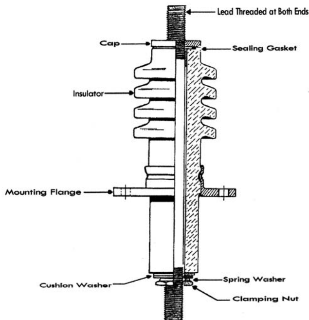
FIGURE 3.2.1 Solid-type bushing.
