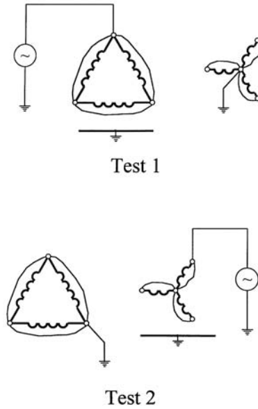
FIGURE 3.6.11 Applied-voltage tests on two-winding transformers.
