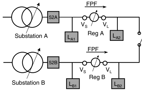
FIGURE 3.7.7A Step-voltage regulator in routine application.
