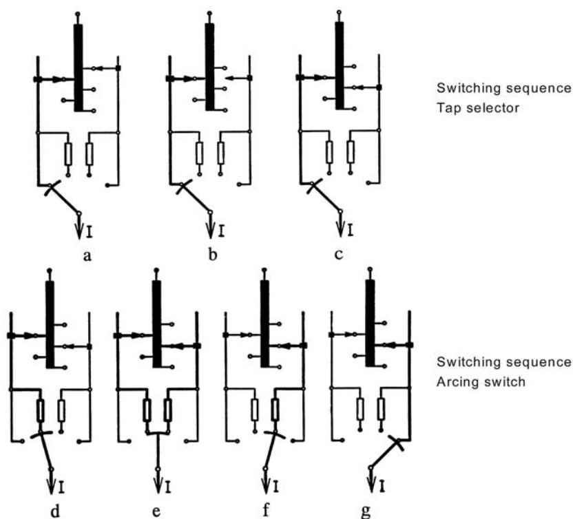
FIGURE 3.3.2 Switching sequence of tap selector — arcing switch.
