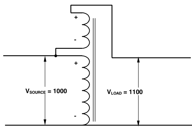
FIGURE 2.7.13 Step-up autotransformer.
