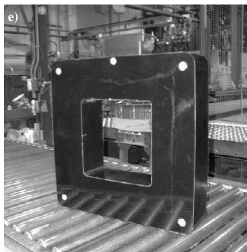
FIGURE 2.6.20 (a) Small 600-V-class window-type CT mounted over a bushing on a 15-kV recloser. (b) 15-kV-class window-type CTs with porcelain sleeve mounted on substation structure. (c) 600-V-class window-type CTs mounted over a 15-kV bus inside a metal enclosure. (d) Large 600-V-class window-type CT (slipover) mounted over a high-voltage bushing. (e) 8.7-kV-class window-type CT with rectangular opening. (Photos courtesy of Kuhlman Electric Corp.)
