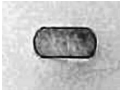
FIGURE 2.2.4 Cross section of enameled round wire after flattening. (By permission of ABB Inc., Jefferson City, MO. )
