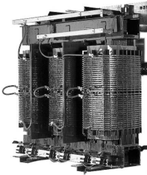
FIGURE 2.5.2 Three-phase 1500-kVA dry-type transformer, 15-kV-class primary, 600-V secondary. Three cooling fans can be seen on the base, below the coils. (Photo courtesy of ABB.)
