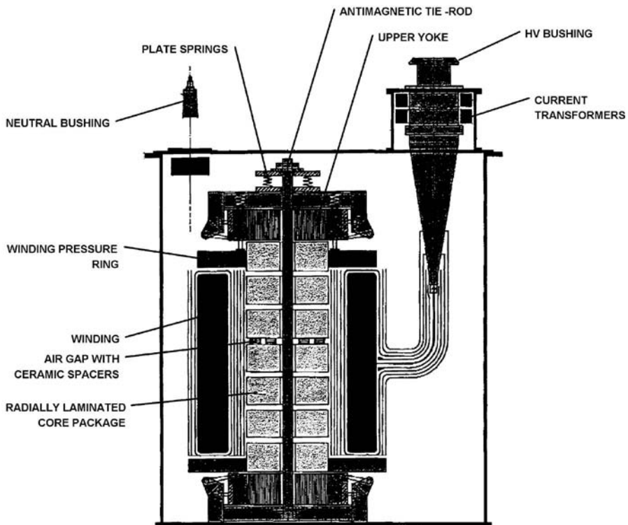
FIGURE 2.9.3 Gapped iron-core oil-immersed reactor.
