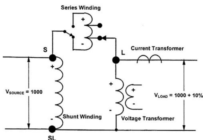
FIGURE 2.7.23 Voltage regulation on the load side (Type A).
