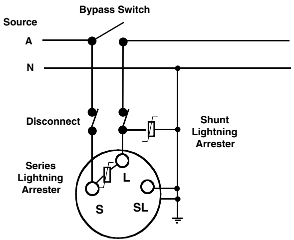
FIGURE 2.7.3 Voltage regulator connection in a single-phase circuit.
