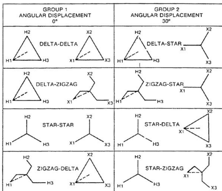
FIGURE 3.5.2 Standard angular displacement for three-phase transformers.
