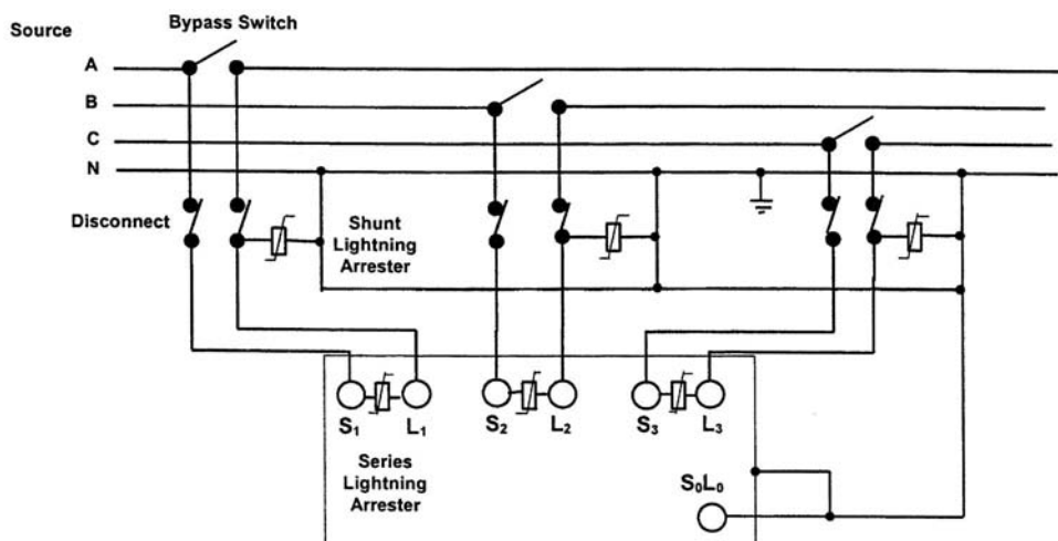
FIGURE 2.7.26 Connection of three-phase regulator regulating a three-phase, four-wire, multigrounded wye circuit.
