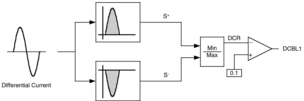
FIGURE 3.8.15 DC blocking logic.
