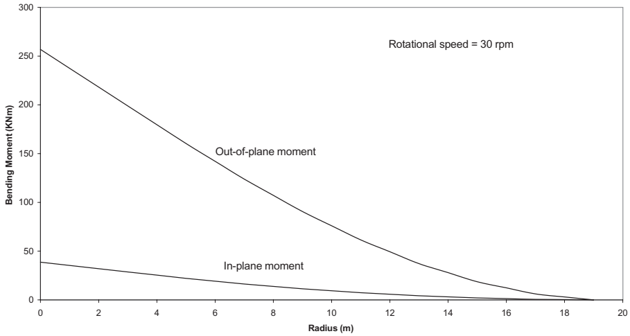
Figure 5.7 Blade In-plane and Out-of-plane Aerodynamic Bending Moment Distributions for Typical 40 m Diameter Stall-regulated Machine Operating in a Steady, Uniform 10 m/s Wind
