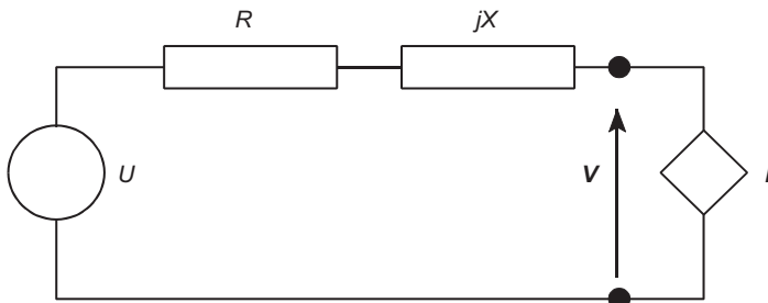
Figure 10.18 Use of 'Fictitious Grid' to Establish Voltage Variations for Various Potential Networks ( I – measured current (complex quantity), R – resistance of fictitious grid, jX – inductive reactance of fictitious grid, U – ideal source voltage, V – synthesized voltage |V| passed through flicker algorithm)
