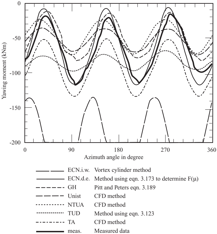
Figure 3.73 Yawing Moment on the Tjæreborg Turbine at 32° Yaw and 8.5 m/s, (Snel and Schepers 1995)
