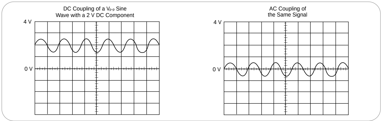
► Figure 23. AC and DC input coupling.
