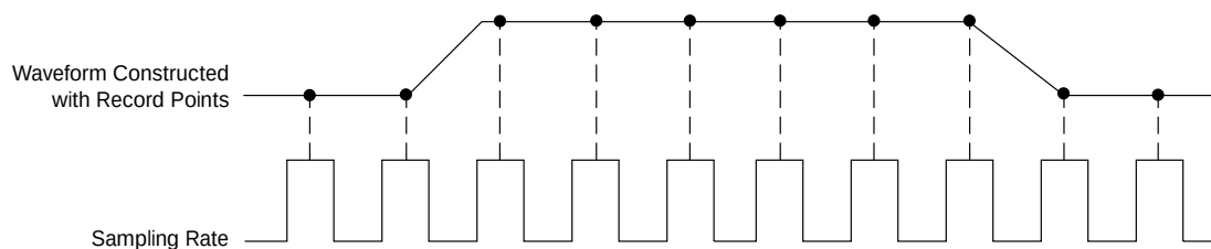
► Figure 29. Real-time sampling method.
