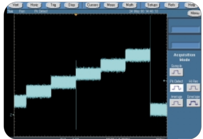
► Figure 27. Peak detect mode enables the TDS7000 Series oscilloscope to capture transient anomalies as narrow as 100 ps.
