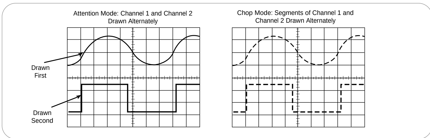
► Figure 24. Multi-channel display modes.
