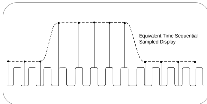
► Figure 34. In sequential equivalent-time sampling, a single sample is taken for each recognized trigger after a time delay which is incremented after each cycle.
