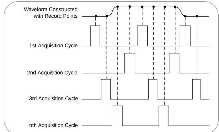
► Figure 32. Some oscilloscopes use equivalent-time sampling to capture and display very fast, repetitive signals.
