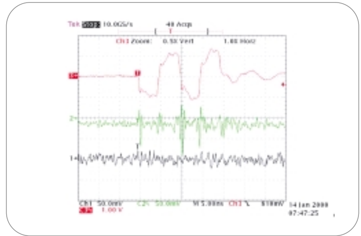
► Figure 43. Differential probes can separate common-mode noise from the signal content of interest in today's fast, low-voltage applications – especially important as digital signals continue to fall below typical noise thresholds found in integrated circuits.
