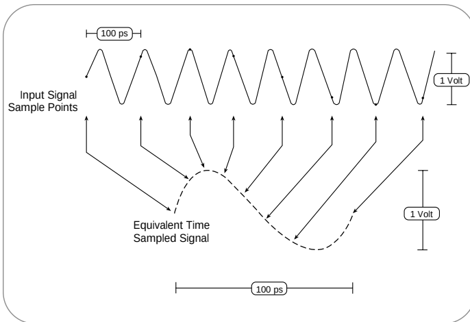
► Figure 28. Basic Sampling. Sampled points are connected by interpolation to produce a continuous waveform.
