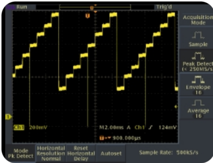
▶ Figure 25. Example of an acquisition menu.
