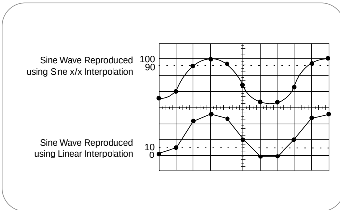
► Figure 31. Linear and sin x/x interpolation.
