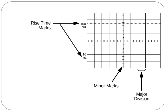
► Figure 38. An oscilloscope graticule.
