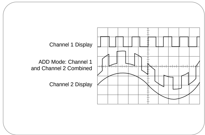
► Figure 39. Adding channels.
