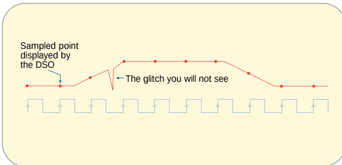
► Figure 26. Sample rate varies with time base settings – the slower the time base setting, the slower the sample rate. Some digital oscilloscopes provide peak detect mode to capture fast transients at slow sweep speeds.
