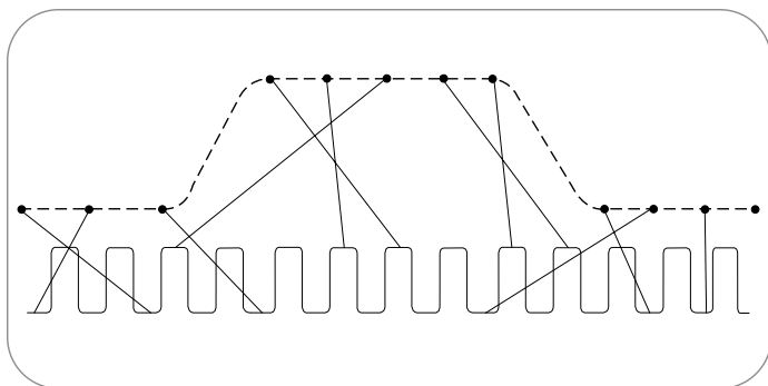
► Figure 33. In random equivalent-time sampling, the sampling clock runs asynchronously with the input signal and the trigger.
