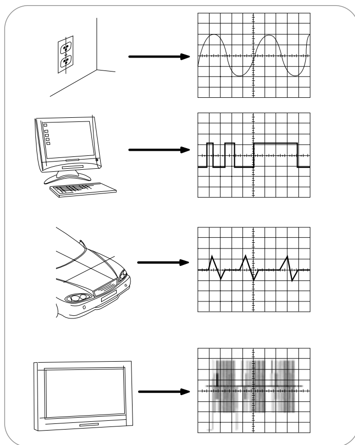
► Figure 4. Sources of common waveforms.
