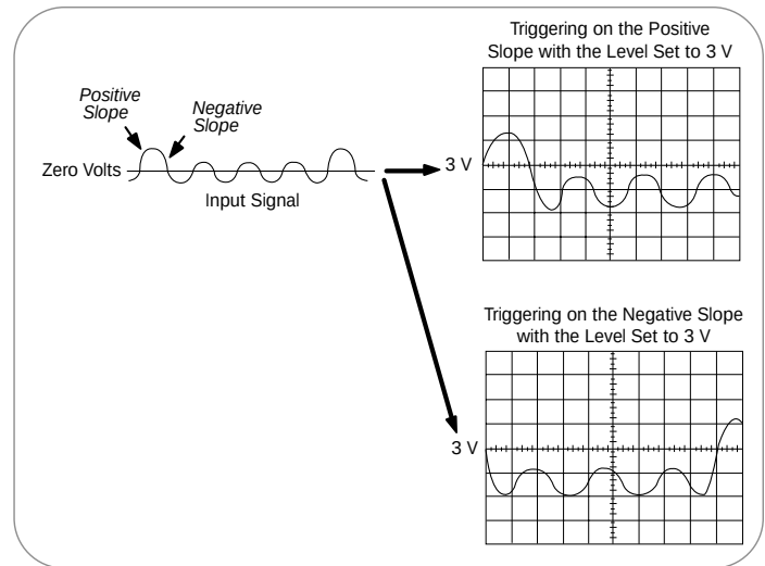
► Figure 36. Positive and negative slope triggering.
