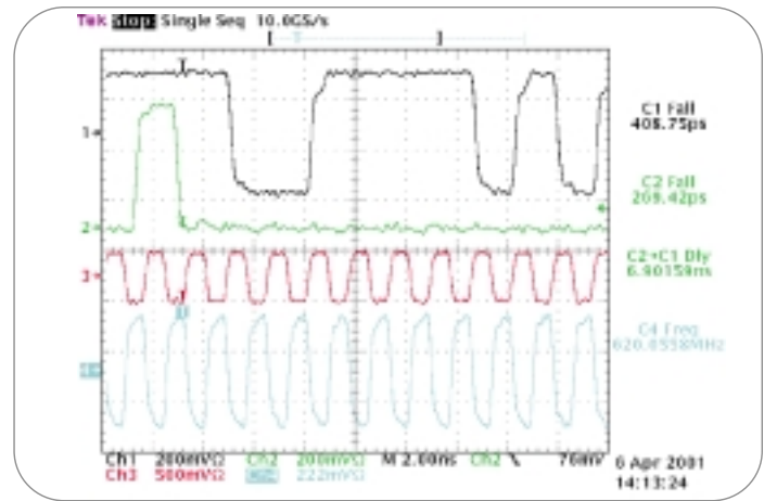
► Figure 17. The TDS694C delivers high-speed, single-shot acquisition across multiple channels, increasing the likelihood of capturing elusive glitches and transient events.
