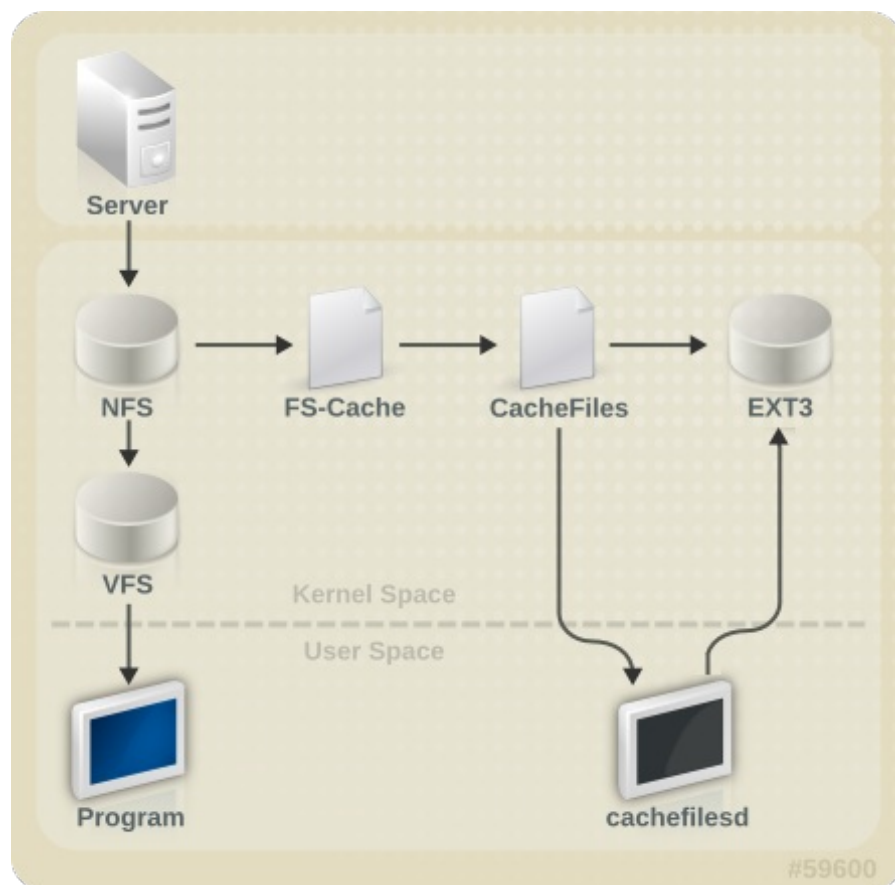
Figure 9.1. FS-Cache Overview
